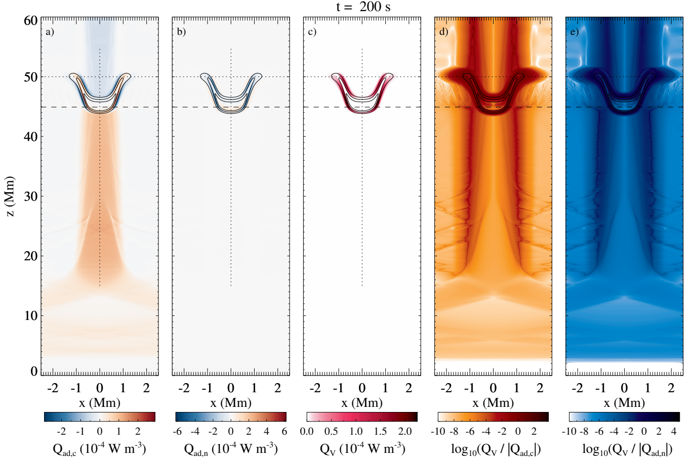
Figure A6: Comparison between adiabatic and frictional heatings. Panels a ) and b ) represent the adiabatic variation of internal energy of the charged and the neutral fluids, Q_{\text{ad},c} and Q_{\text{ad},n} , respectively. Panel c ) shows the frictional heating due to collisions. Panels d ) and e ) represent the ratios between the frictional heating and the absolute values of Q_{\text{ad},c} and Q_{\text{ad},n} , respectively.
