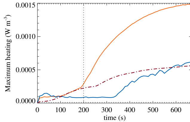
Figure A7: Maximum values of the heating terms as functions of time. Orange and blue solid lines correspond to the maximum values of the adiabatic heating of the charged and the neutral fluid, respectively. The dotted-dashed line represent the results for the frictional heating due to charged-neutral collisions. The vertical dotted line shows the time of the simulation represented in Fig. 6.
