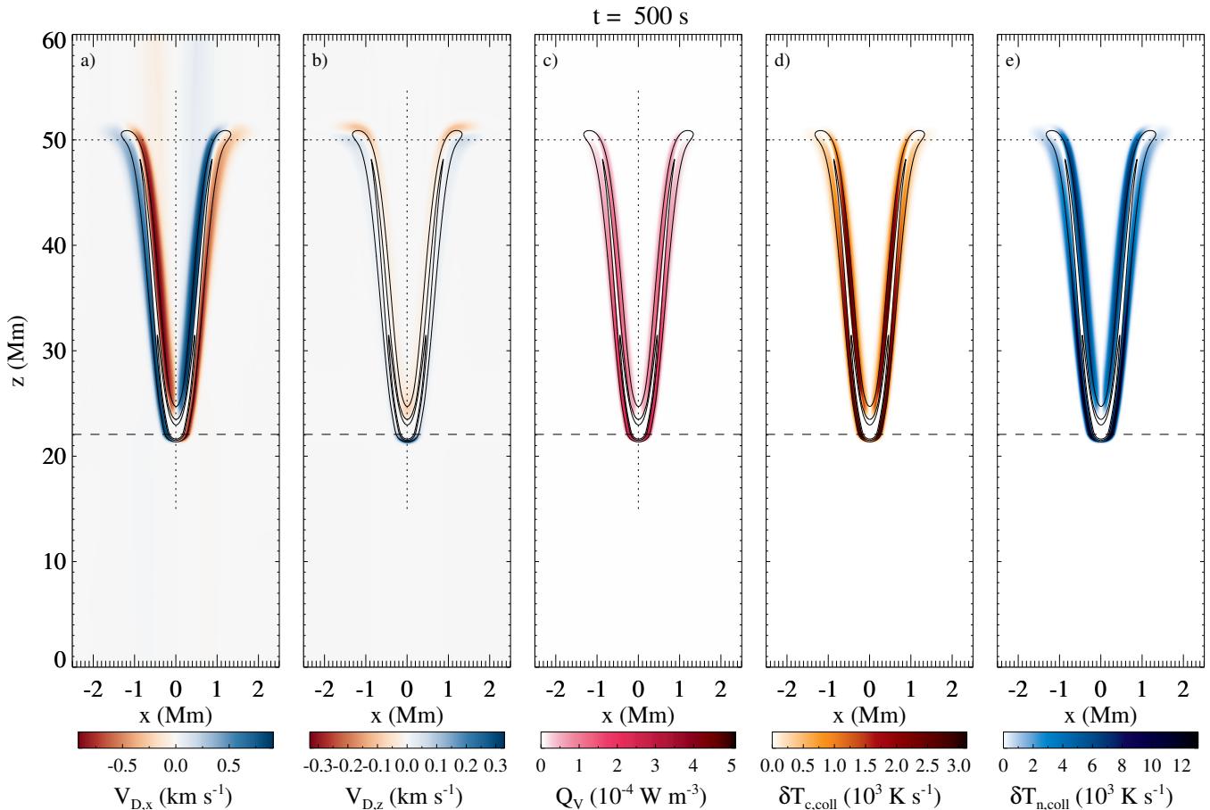
Figure 2. Snapshot of the simulation of a falling coronal rain blob. a) and b) : color maps of the x -component and z -component of the drift velocity, V_{D,x} and V_{D,z} , respectively; c) : color map of the frictional heating, Q_V ; d) and e) : color maps of the temperature variations of the charged and the neutral fluid, respectively, caused by the frictional heating represented in c) . Black solid lines represent density contours of the neutral fluid. A vertical dotted line has been drawn at x = 0 and two horizontal dashed and dotted lines have been drawn at the maximum density and initial blob positions, respectively. (An animation of this figure is available online. The animation runs for a total real-time of 660 s. It shows the evolution of the variables presented in the figure and how the initial Gaussian profile of the blob, given by Eq. (10) develops into a V-shape as the plasma falls down.)
