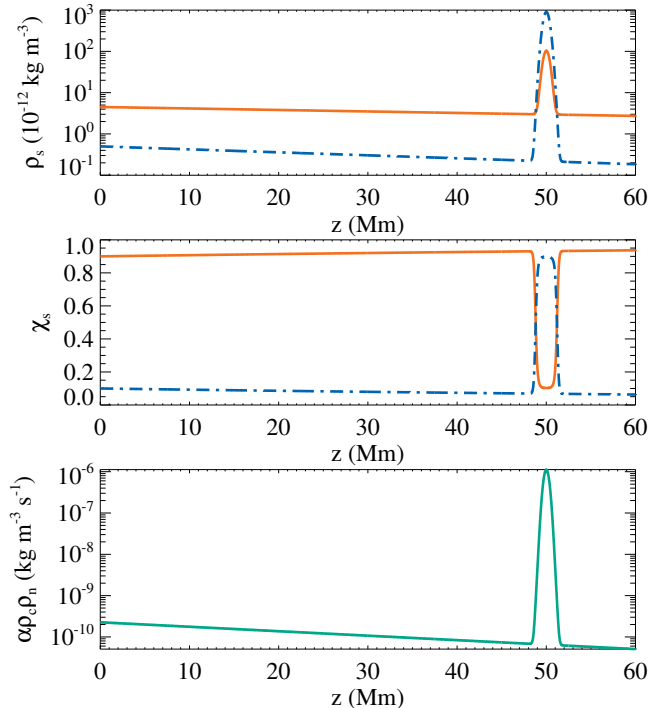
Figure 1. Sketch of the initial time of the simulation. Top and middle panels show the densities, \rho_s , and the relative abundances, \chi_s , of the charged and neutral fluids, represented by orange solid lines and blue dashed-dotted lines, respectively. Bottom panel shows the collisional coupling degree between the two fluids, given by the term \alpha\rho_c\rho_n .
